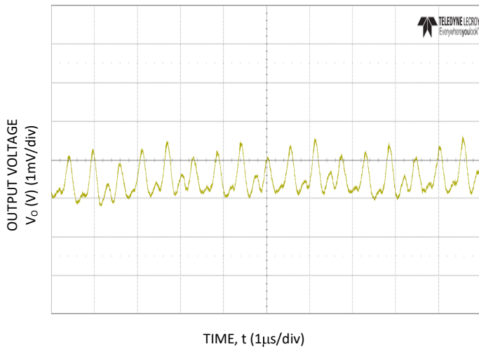
Figure 9. Typical output ripple (C o =4x0.047μF + 4x0.1μF + 15x22μF + 73x47μF + 6x470μF polymer, V IN = 12V, I o = I o,max ).
