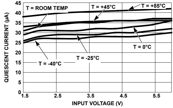
FIGURE 2. QUIESCIENT CURRENT vs INPUT VOLTAGE ( V_{OUT} = 1.85V )
