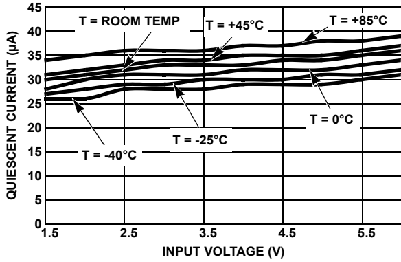
FIGURE 1. QUIESCIENT CURRENT vs INPUT VOLTAGE ( V_{OUT} = 0.9V )
