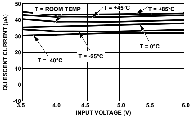
FIGURE 3. QUIESCIENT CURRENT vs INPUT VOLTAGE ( V_{OUT} = 3.3V )
