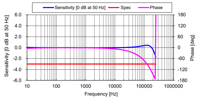
Figure 7: Frequency response
