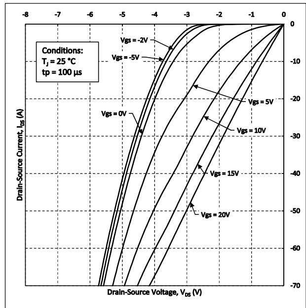
Figure 10. Freewheeling Diode Characteristics at T_J = 25^\circ\text{C}
