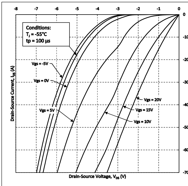
Figure 9. Freewheeling Diode Characteristics at T_J = -55^\circ\text{C}
