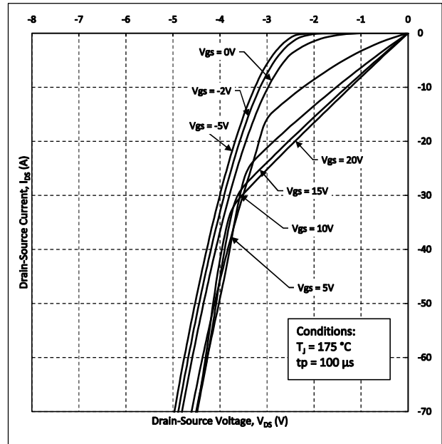
Figure 12. Freewheeling Diode Characteristics at T_J = 175^\circ\text{C}
