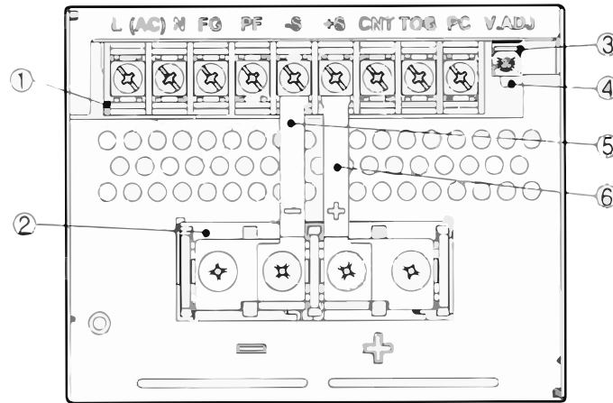
① TB1 Terminal Block (Screw M3 5X8)
