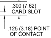
SINGLE ROW CONTACTS READ ONE SIDE OF DAUGHTER BOARD
