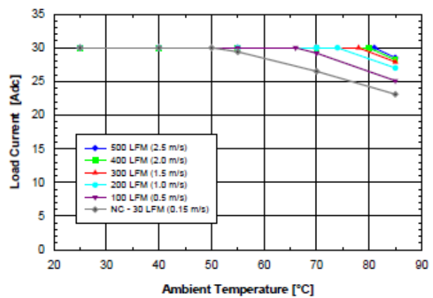
Fig. 1.2V.2: Available load current vs. ambient air temperature and airflow rates for SQE48T30012 converter mounted horizontally with air flowing from pin 3 to pin 1, MOSFET temperature \leq 120 °C, Vin = 48 V.
