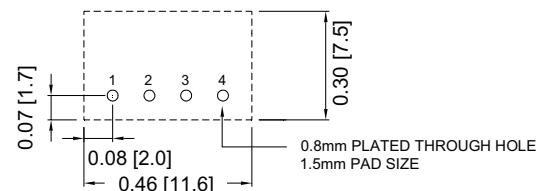
Recommended PCB Layout Top View
