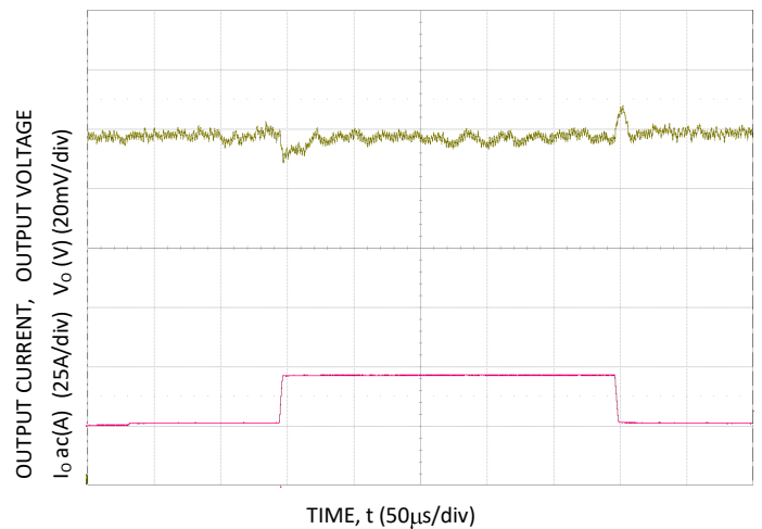
Figure 22. Trans. Resp. to 10A/µs Load Change from 25% to 75% at 12V IN , C_o = 4 \times 0.047\mu\text{F} + 4 \times 0.1\mu\text{F} + 15 \times 22\mu\text{F} + 73 \times 47\mu\text{F} + 6 \times 470\mu\text{F} polymer
