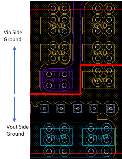
Figure 30. Example of split input-output ground
