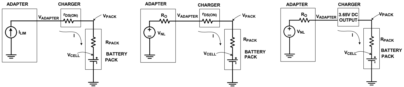
FIGURE 28A. THE EQUIVALENT CIRCUIT IN THE CONSTANT CURRENT REGION FIGURE 28B. THE EQUIVALENT CIRCUIT IN THE RESISTANCE-LIMIT REGION FIGURE 28C. THE EQUIVALENT CIRCUIT WHEN THE PACK VOLTAGE REACHES THE FINAL CHARGE VOLTAGE
