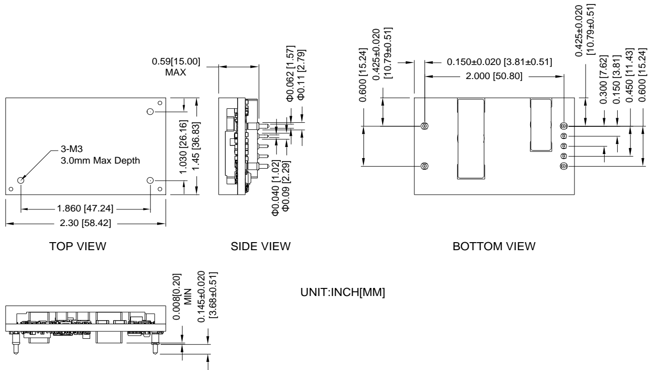
Figure 52. ORQB-50Y24L/0 Outline
