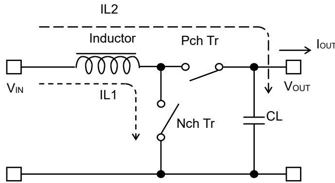
Basic Circuit
