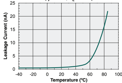
Leakage Current vs. Temperature Measured Across Pins 5&6 & 7&8 ( I_F=0mA, V_L=280V )
