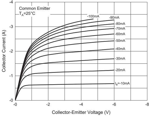
Fig. 1 - Static Characteristics
