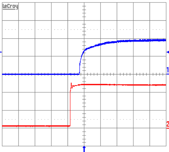
Figure 4. V_{in} versus output voltage for SQE48T30010 converter mounted horizontally. V_{in}=48V_{dc} , I_{out}=30 Amps and turned on using V_{cc} . Top trace: Output voltage (0.5 V/div.). Bottom trace: VCC (20 V/div.). Time scale: 2 ms/div. Convection cooled with T_a=25^{\circ}C .
