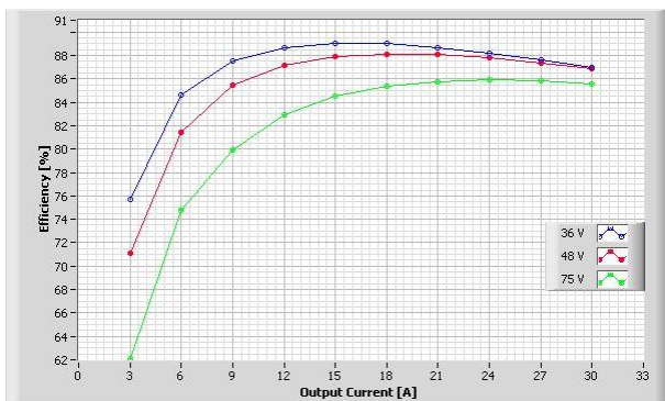
Figure 2. Efficiency vs. load current and input voltage for SQE48T30010 converter mounted horizontally. Convection cooled with T_a = 25\text{ }^\circ\text{C} .
