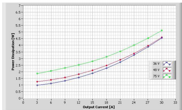
Figure 3. Power dissipation vs. load current and for SQE48T30010 converter mounted horizontally. Convection cooled with T_a = 25\text{ }^\circ\text{C} .
