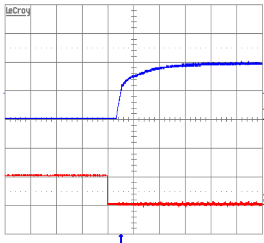
Figure 7. Turn-on transient at full rated load current (resistive) plus 10,000 \mu F at V_{in} = 48 V, 30 Amps and turned on using ON/OFF pin. Top trace, I_{out} =Output voltage (0.5 V/div.). Bottom trace: ON/OFF signal (5 V/div.). Time scale: 2 ms/div.
