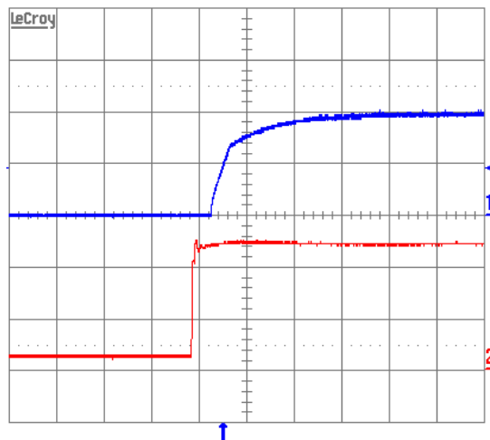
Figure 5. V_{in} versus output voltage for SQE48T30010 converter mounted horizontally. V_{in}=48V_{dc} , I_{out}=30 Amps, C_{out}=10,000\mu F and turned on using V_{cc} . Convection cooled with T_a=25^{\circ}C . Top trace: Output voltage (0.5 V/div.). Bottom trace: VCC (20 V/div.). Time scale: 2 ms/div. Convection cooled with T_a=25^{\circ}C .
