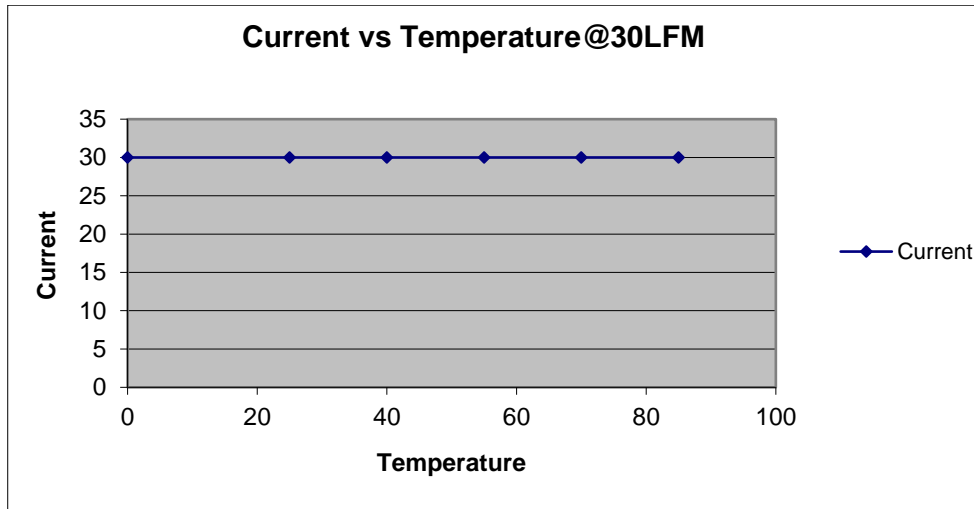
Figure 1. Available load current vs. ambient air temperature for an SQE48T30010 converter mounted vertically with air flowing from pin 3 to pin 1, MOSFET temperature \leq 125\text{ }^\circ\text{C} , V_{in} = 48\text{ V} .
