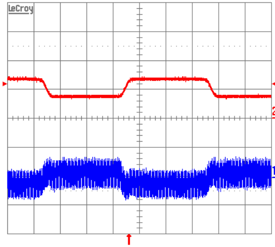
Figure 8. Output voltage response to load current step-change (7.5A – 15A – 7.5A) at V_{in} = 48\text{ V} . Top trace: load current (5 A/div.) Bottom trace: output voltage (50 mV/div.). Current slew rate: 0.1 A/ \mu\text{s} . C_o = 1\ \mu\text{F} ceramic. Time scale: 0.1 ms/div.
