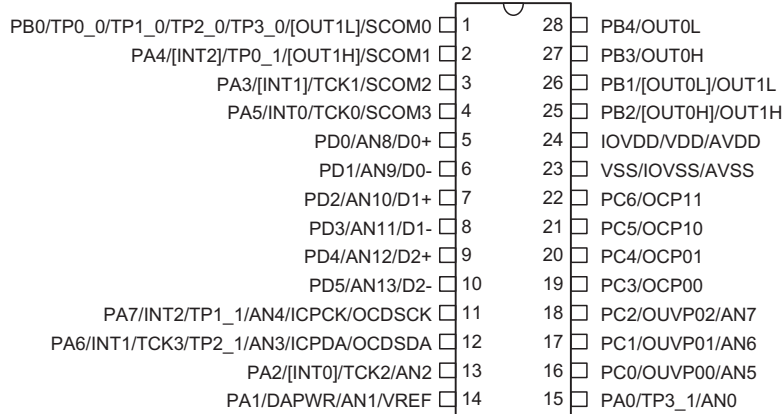
HT45V4N 28 SSOP-A
