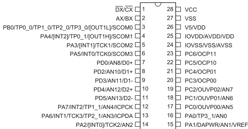
HT45FH4N 28 SSOP-A
