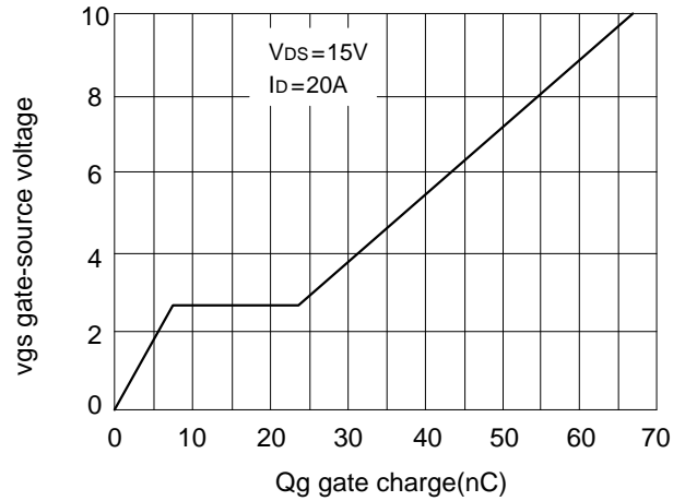
Fig.4 gate charge
