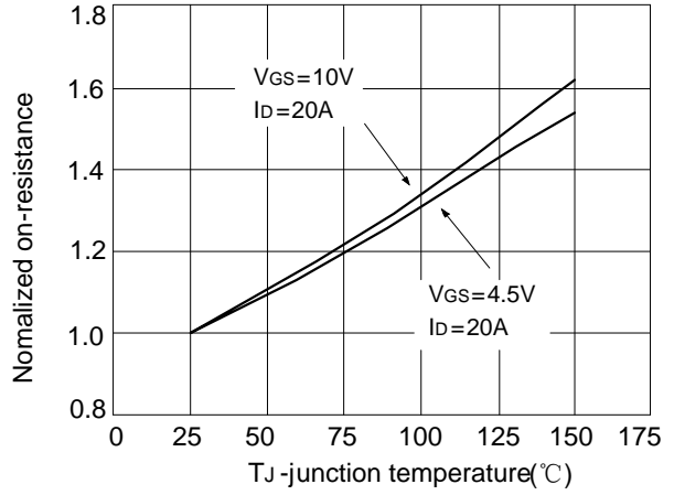
Fig.2 rdson-junction temperature
