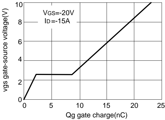
Fig.9 gate charge
