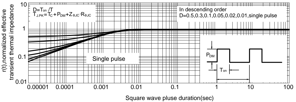
Fig.11 normalized maximum transient thermal impedance
