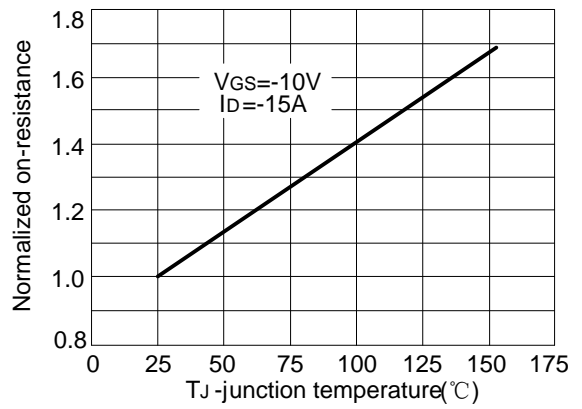
Fig.4 drain-source on-resistance
