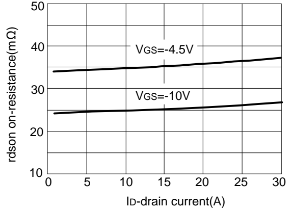
Fig.2 drain-source on-resistance
