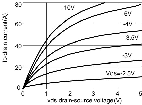
Fig.3 output characteristics
