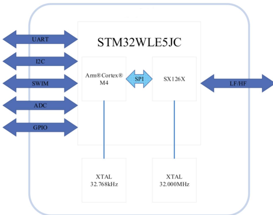
Figure 1 LoRa-E5 Schematic diagram
