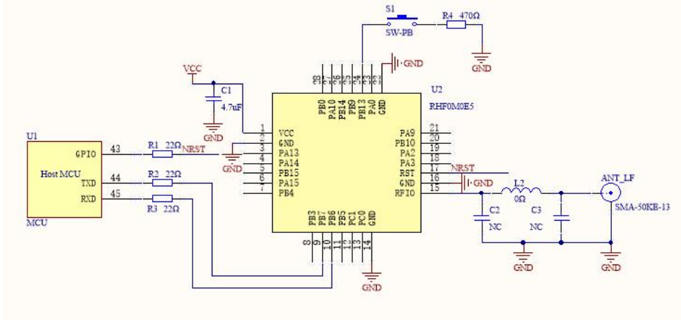
Figure 12 Reference design based on LoRa-E5
