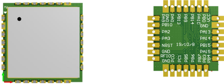
Figure 16 RHF0M0E5 Module appearance
