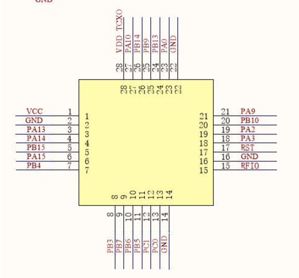
Figure 2 LoRa-E5 Pin arrangement
