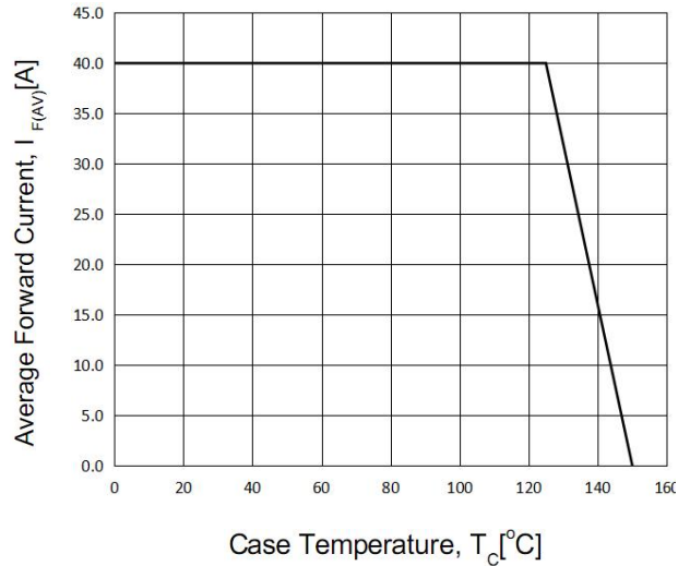
Figure 4. Power Derating
