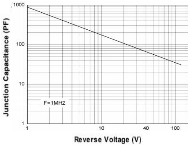
Figure 3. Junction Capacitance
