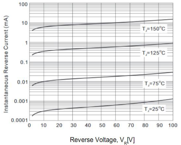
Figure 2. Reverse Leakage Current
