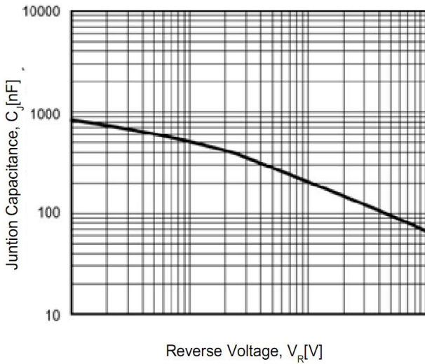
Figure 3. Junction Capacitance
