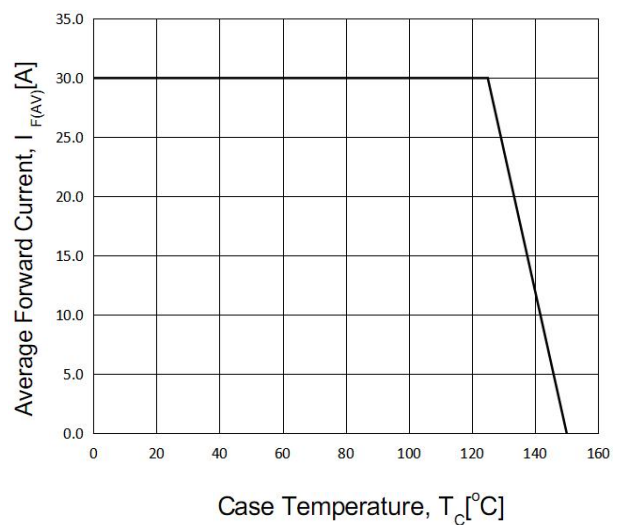
Figure 4. Power Derating
