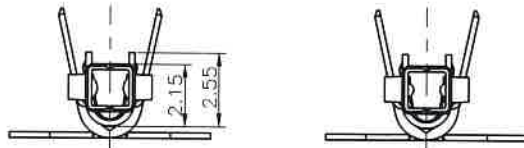
CONTACT DIMPLE CONFIGURATIONS 接触点配置
