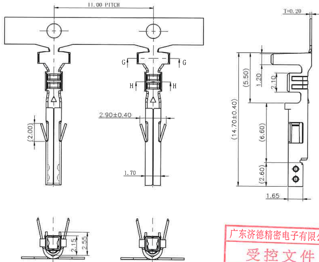
CONTACT DIMPLE CONFIGURATIONS 接触点配置
