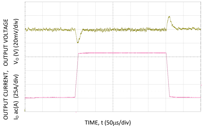
Figure 10. Trans. Resp. to 100A/μs Load Change from 25% to 75% at 12V IN , C o =4x0.047μF + 4x0.1μF + 15x22μF + 73x47μF + 6x470μF polymer
