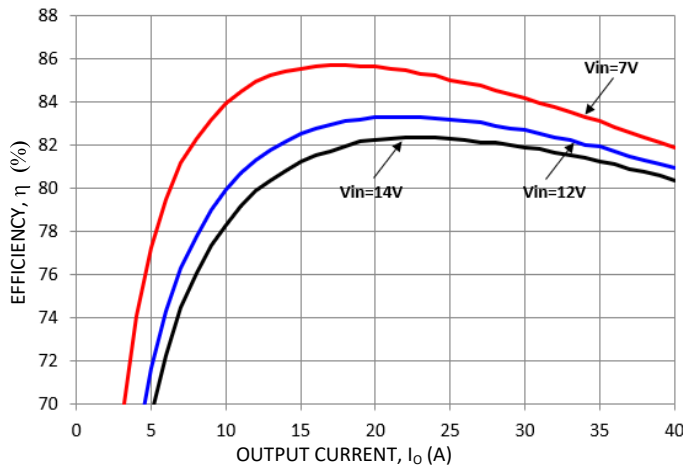
Figure 1. Converter Efficiency versus Output Current.
