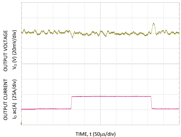
Figure 4. Trans. Resp. to 10A/μs Load Change from 25% to 75% at 12V IN , C_o=4 \times 0.047 \mu\text{F} + 4 \times 0.1 \mu\text{F} + 15 \times 22 \mu\text{F} + 73 \times 47 \mu\text{F} + 6 \times 470 \mu\text{F} polymer
