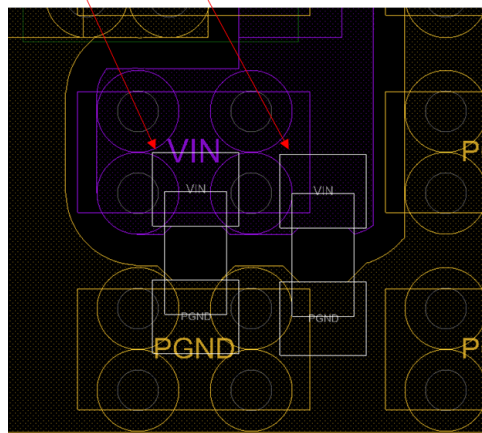
Figure 31. Example of Input capacitor placement and routing
