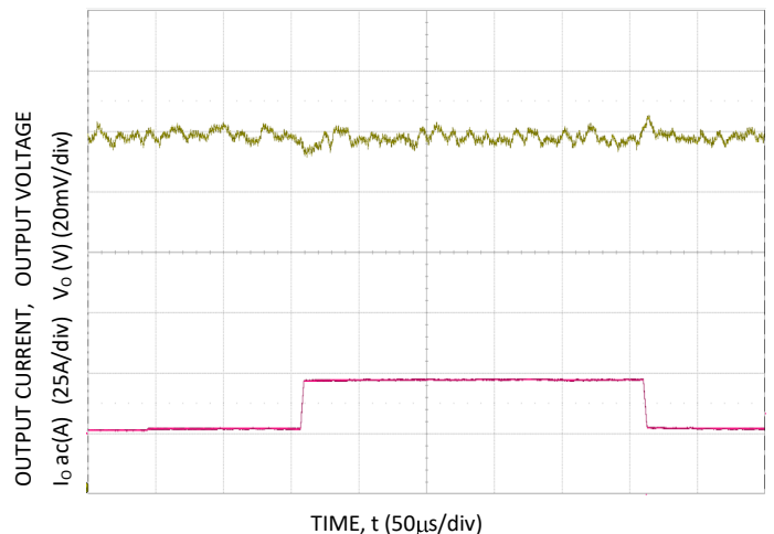
Figure 22. Trans. Res. to 10A/µs Load Change from 25% to 75% at 12V IN , C_o=4 \times 0.047\mu\text{F} + 4 \times 0.1\mu\text{F} + 15 \times 22\mu\text{F} + 73 \times 47\mu\text{F} + 6 \times 470\mu\text{F} polymer
