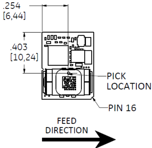
Pick and Place Location
