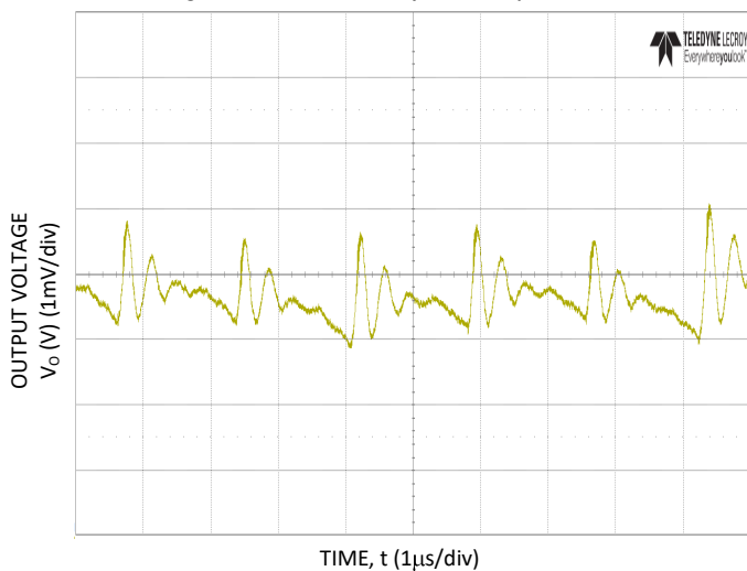
Figure 3. Typical output ripple ( C_o=4 \times 0.047 \mu\text{F} + 4 \times 0.1 \mu\text{F} + 15 \times 22 \mu\text{F} + 73 \times 47 \mu\text{F} + 6 \times 470 \mu\text{F} polymer, V_{IN} = 12\text{V} , I_o = I_{o,max} ).
