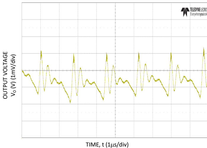
Figure 9. Typical output ripple (C o =4x0.047μF + 4x0.1μF + 15x22μF + 73x47μF + 6x470μF polymer, V IN = 12V, I o = I o,max ).
