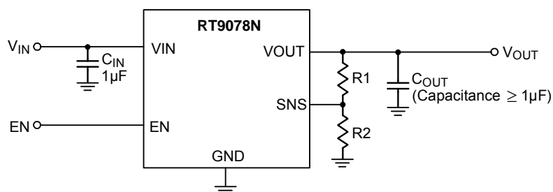
Figure 3. Adjustable Output Voltage Application Circuit
