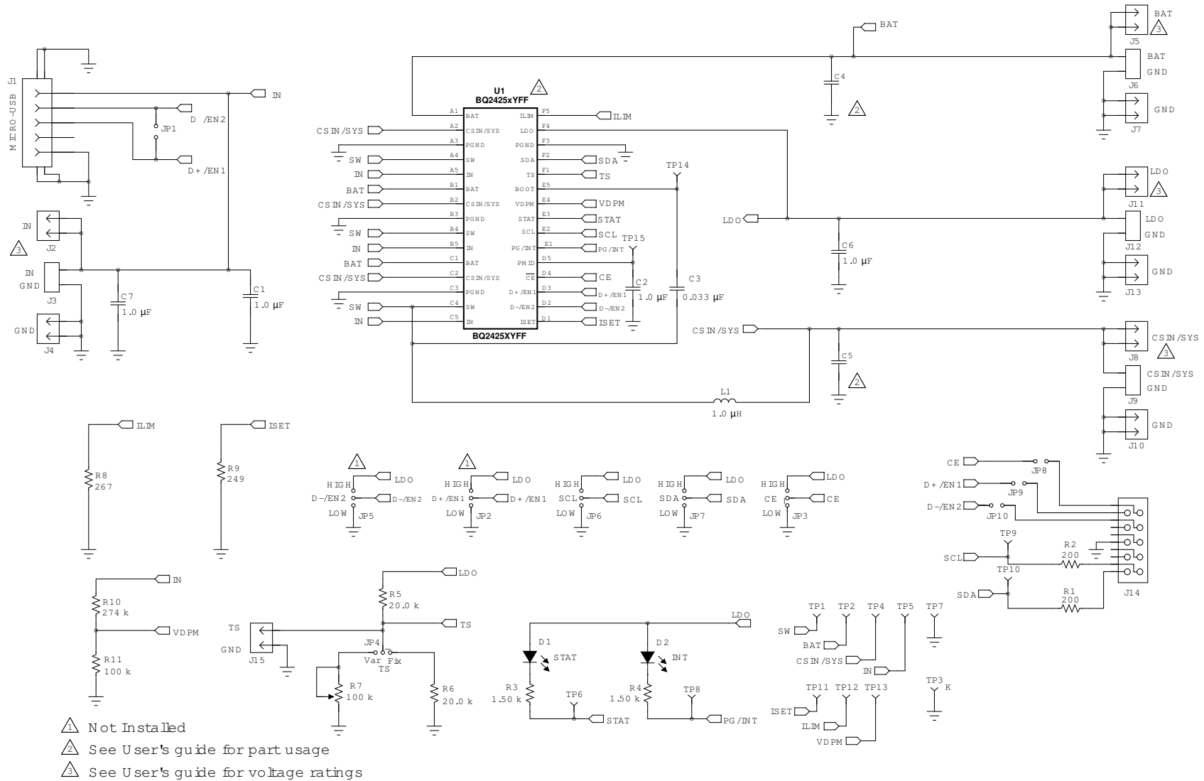
Figure 1. bq2425xEVM-150 Schematic
