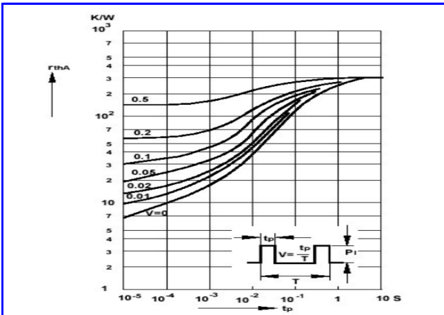
Fig.5-Pulse thermal resistance versus pulse duration
