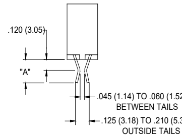
CONTACT CODE 555 BEND USES WIRE HOLE CONTACTS
