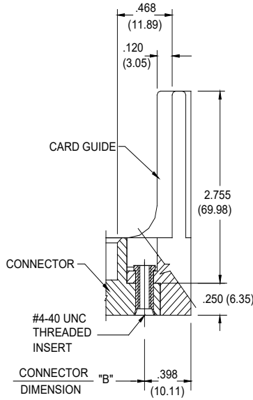
MOUNTING OPTION CODES x58 (OFFSET CARD GUIDES)
