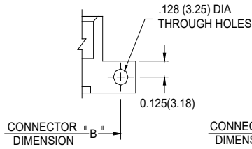
MOUNTING OPTION CODE x12 (SIDE MOUNTING HOLES) WITH INSERTS: CODES X17 & X18, SEE TABLE
