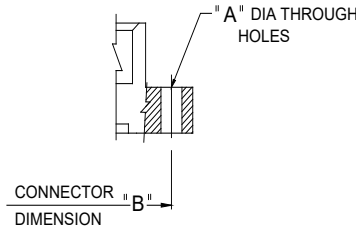
MOUNTING OPTION CODES x02 AND x04 (THROUGH MOUNTING HOLES)
