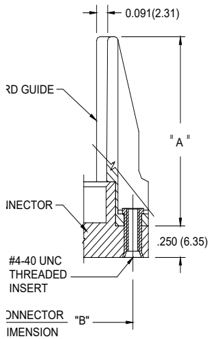
MOUNTING OPTION CODE x78 (IN-LINE CARD GUIDE)
