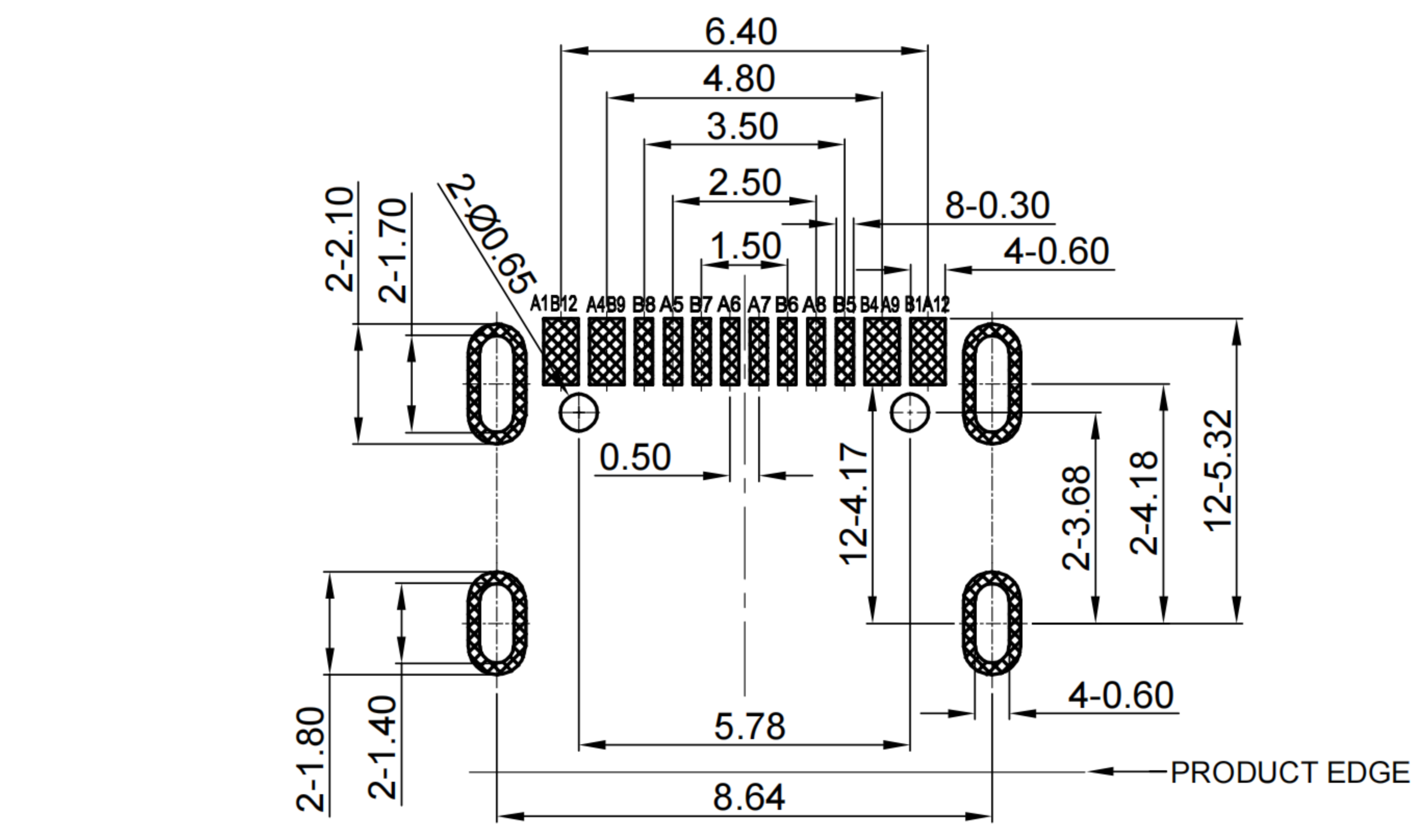
RECOMMENDED P.C.B. LAYOUT TOLERANCE UNSPECIFIED ±0.05mm
