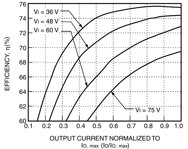
Figure 8. LW005F Typical Efficiency vs. Normalized Output Current at T_c = 25\text{ °C}
