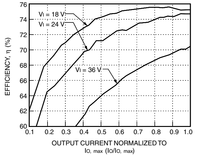
Figure 7. LC005B Typical Efficiency vs. Normalized Output Current at T_c = 25\text{ °C}
