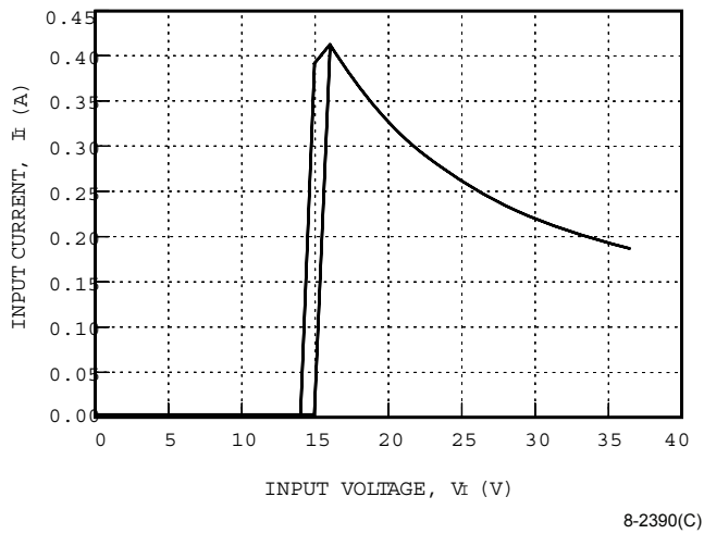
Figure 1. LC005x Input Current vs. Input Voltage at I_o = I_{o,max} and T_c = 25\text{ °C}
