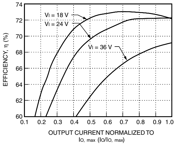
Figure 5. LC005F Typical Efficiency vs. Normalized Output Current at T_c = 25\text{ °C}
