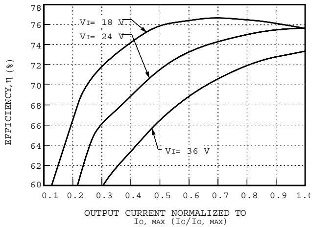
Figure 6. LC005A Typical Efficiency vs. Normalized Output Current at T_c = 25\text{ °C}
