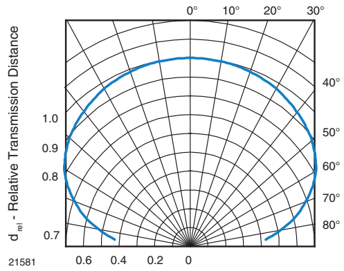
Fig. 11 - Horizontal Directivity
