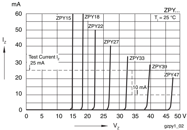
Fig. 7 - Breakdown Characteristics
