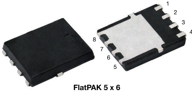
FlatPAK 5 x 6
