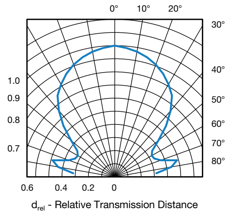
Fig. 11 - Horizontal Directivity
