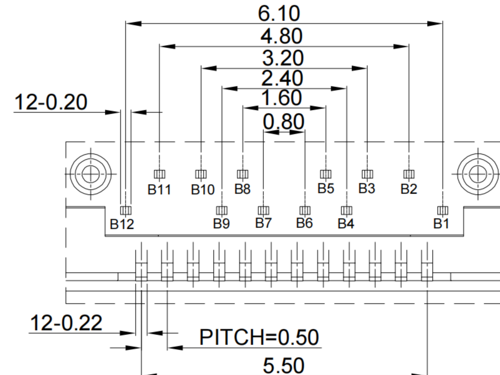
DETAIL A
