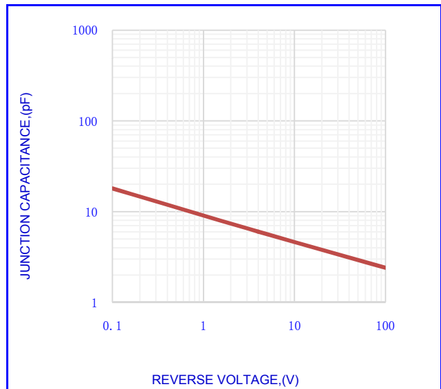
Fig.4-TYPICAL JUNCTION CAPACITANCE
