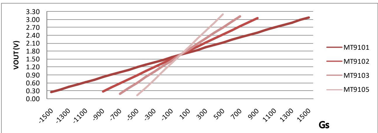
Figure.14 Vout vs. Magnetic Field (At Vcc=3.3V; TA=25°C)
