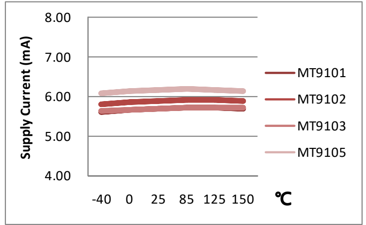
Figure.7 Supply Current vs. Temperature (At Vcc=3.3V)
