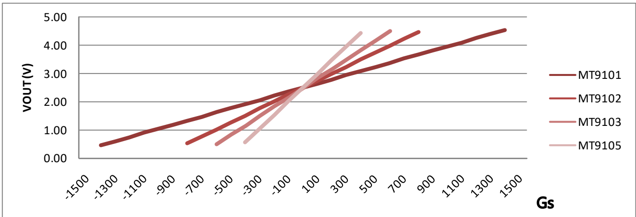
Figure.13 Vout vs. Magnetic Field (At Vcc=5.0V; TA=25°C)
