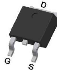
TO-252
