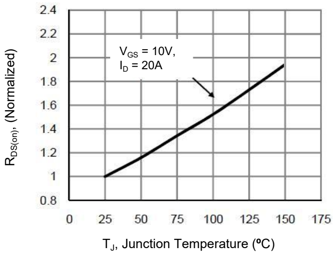
Figure 7. Drain-Source On-Resistance
