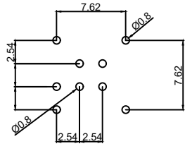
Pcb plate opening size (PCB板开孔尺寸)
