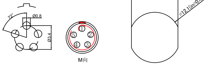
Pcb plate opening size (PCB板开孔尺寸)
