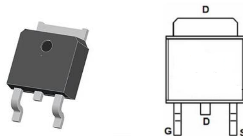
TO-252-2L top view
