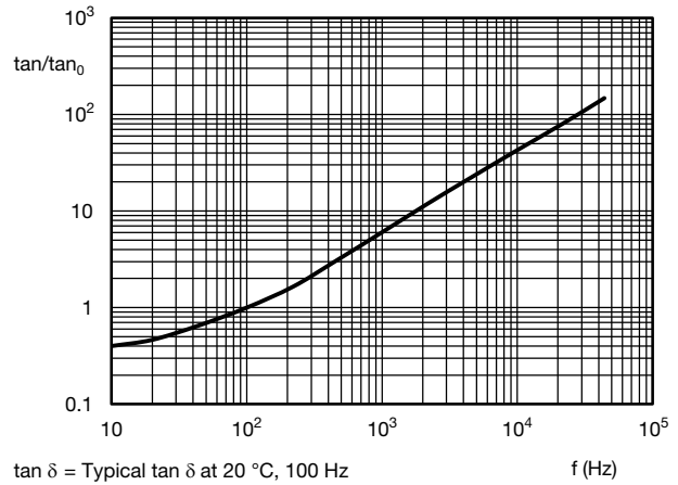
Fig. 10 - Typical multiplier of dissipation factor (tan δ) as a function of frequency
