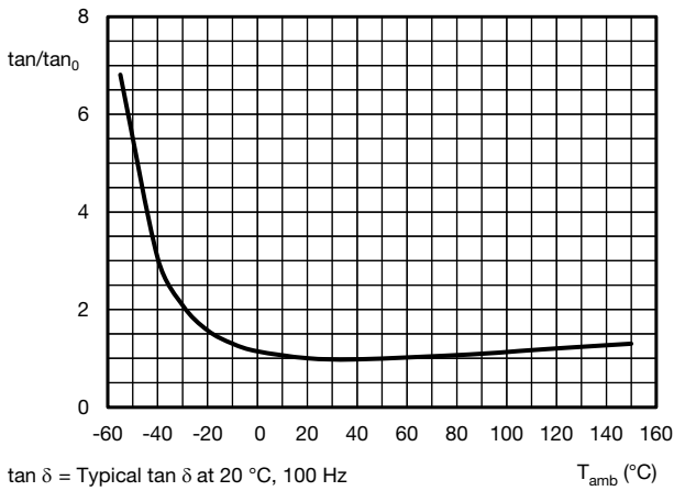
Fig. 9 - Typical multiplier of dissipation factor (tan δ) as a function of ambient temperature
