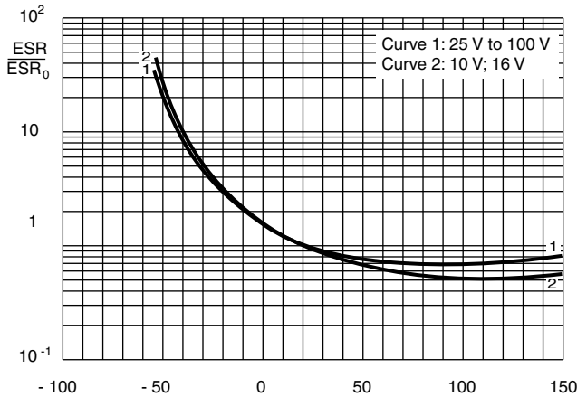
Case \varnothing D \times L = 6.5 \text{ mm} \times 18 \text{ mm} to 15 \text{ mm} \times 30 \text{ mm} ESR_0 = \text{Typical at } 20^\circ\text{C, } 100 \text{ Hz}
