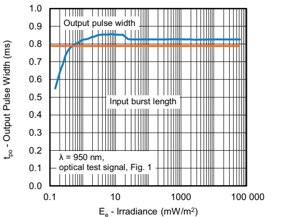
Fig. 2 - Pulse Length and Sensitivity in Dark Ambient
