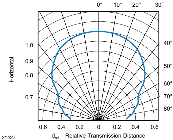
Fig. 11 - Horizontal Directivity
