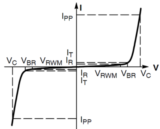
Bi-Directional TVS
