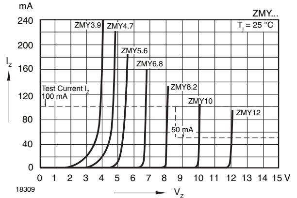
Fig. 5 - Breakdown Characteristics
