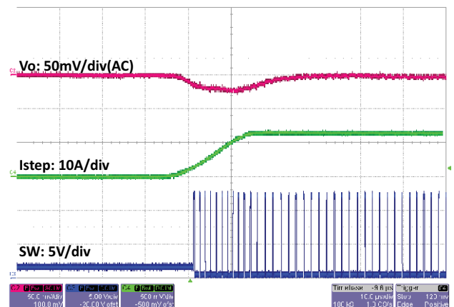
Fig. 38 - SiC451 Load Step, 0 A to 12.5 A, 1 A/ \mu s, t = 10 \mu s/div Skip Mode Enabled
