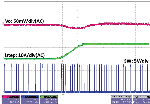
Fig. 34 - SiC451 Load Step, 12.5 A to 25 A, 10 A/ \mu s, t = 10 \mu s/div
