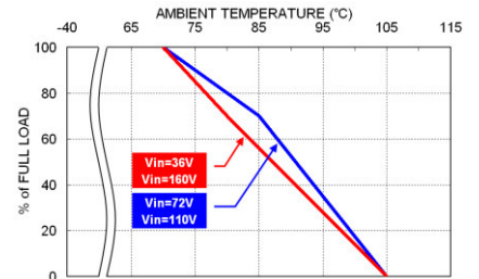
RCD15-110□□□W Derating Curve
